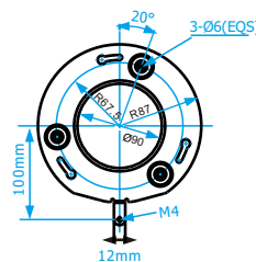
Mounting Plate
